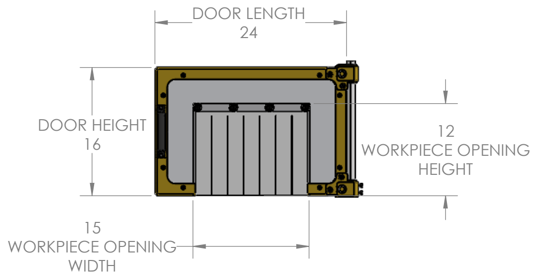
DOORS CLOSED
